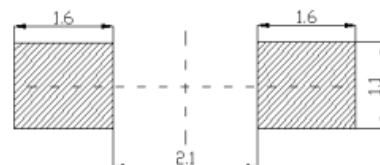
推荐焊盘尺寸 Recommended Soldering Pad
